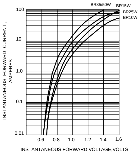
FIG.3-TYPICAL FORWARD CHARACTERISTICS
